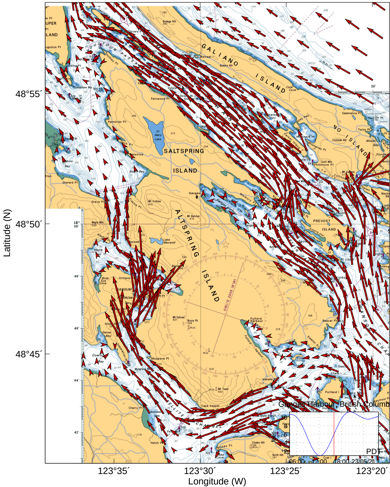
Tidal Currents for Saltspring Island 20-May-2023 16:00:00 [PDT]
