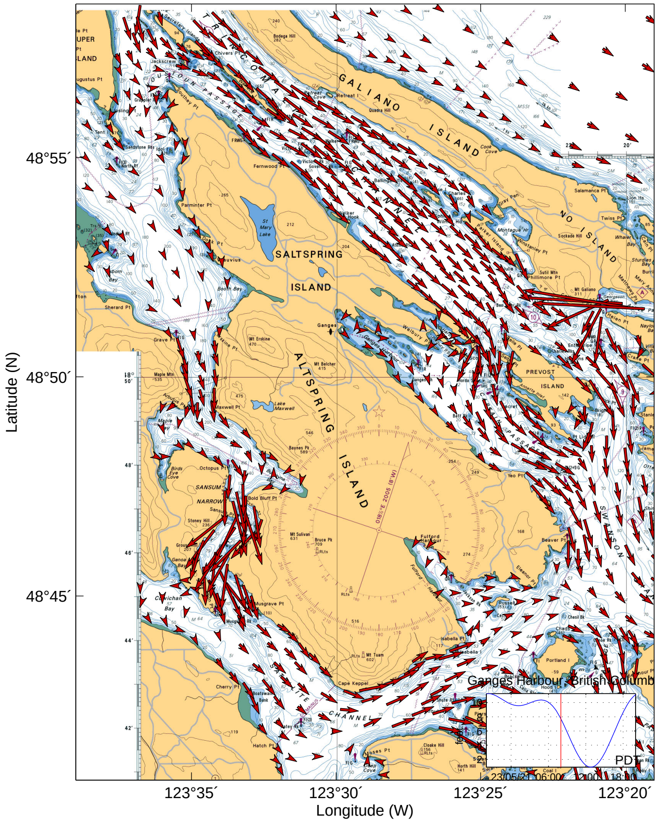
Tidal Currents for Saltspring Island 21-May-2023 08:00:00 [PDT]
