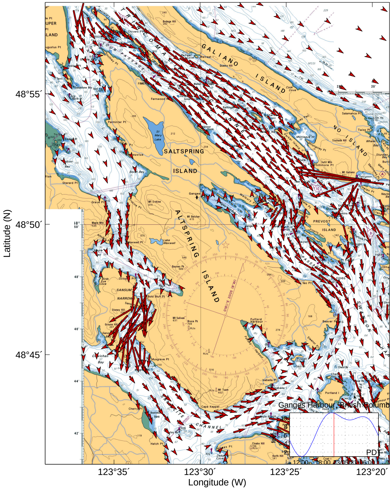
Tidal Currents for Saltspring Island 20-May-2023 21:00:00 [PDT]
